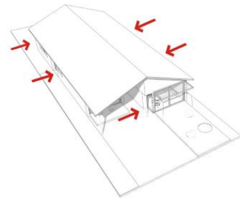
Concept sketches of key principles – design shaped to maximise northern exposure and preserve pleasant outdoor spaces, and various features used to shade windows from the summer sun.
