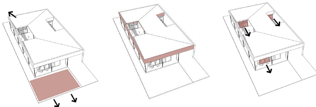
Concept sketches of key principles - northern exposure for pleasant outdoor spaces, various features used to shade windows from the summer sun and courtyards added for maximising solar access
