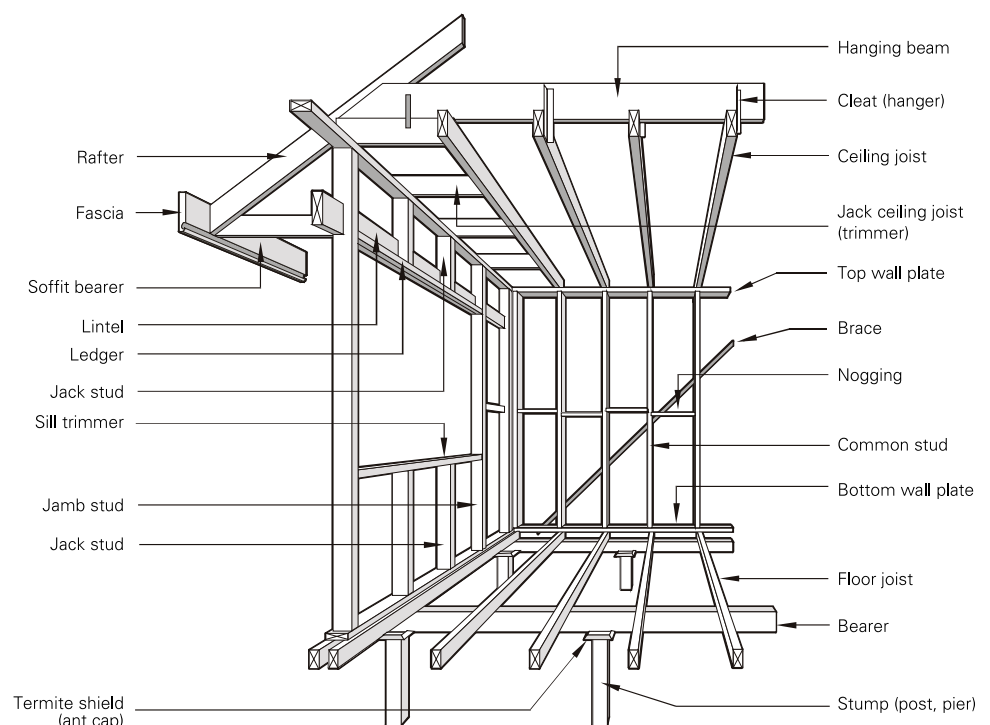
Some terms that apply to timber framing.
